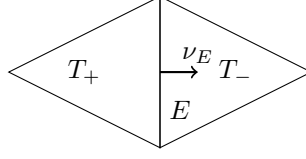
FIGURE 1. Convention for the edge normal.
