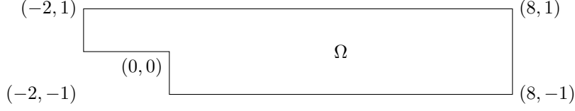
FIGURE 5. The backward facing step.
