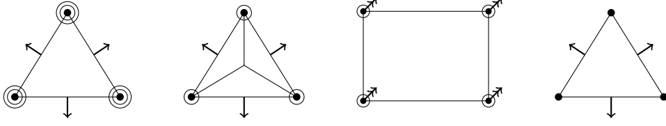
FIGURE 3. Mnemonic diagrams of some finite elements for the bi-harmonic equation: Argyris, HCT, BFS (definitions see [Cia78]), and Morley.
