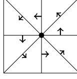
FIGURE 2. Orientation of the normal vectors \hat{\nu}_E around the vertex z
