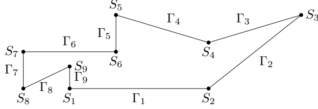
FIGURE 1. Our notation for a polygon.
