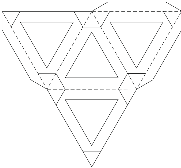
Tetraeder
